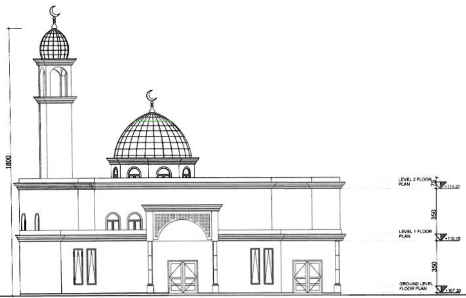
1 NORTH ELEVATION SP102
