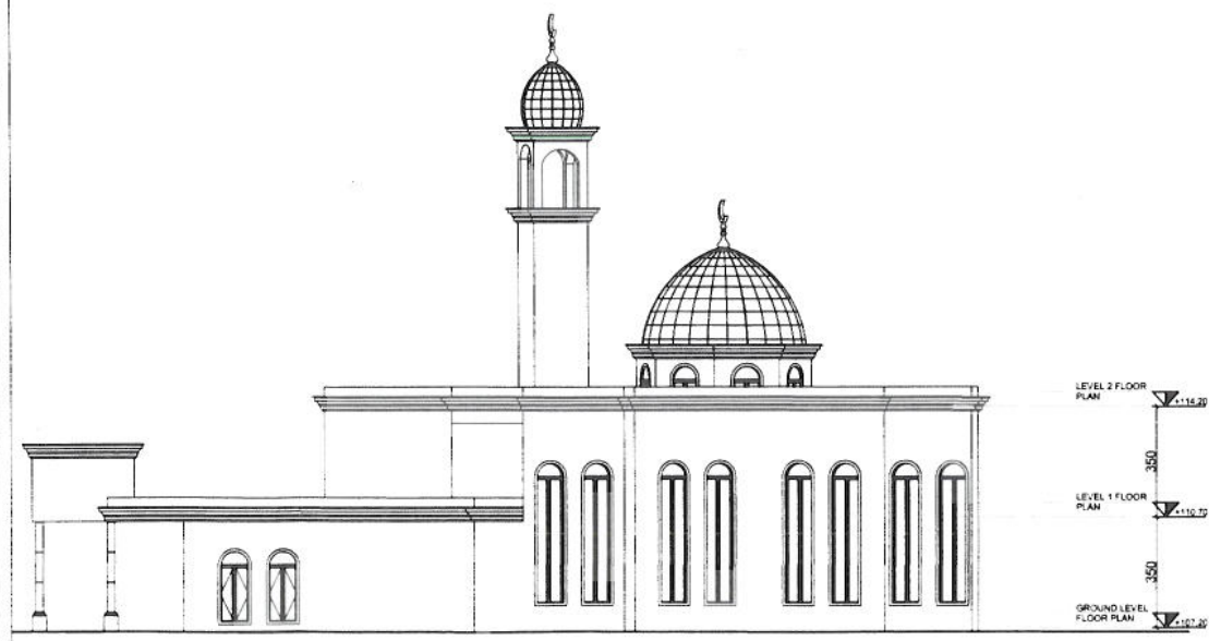
4 WEST ELEVATION SP102
