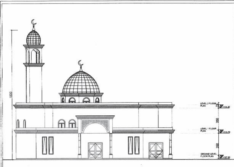
1 NORTH ELEVATION
