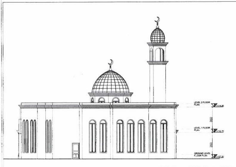
3 SOUTH ELEVATION
