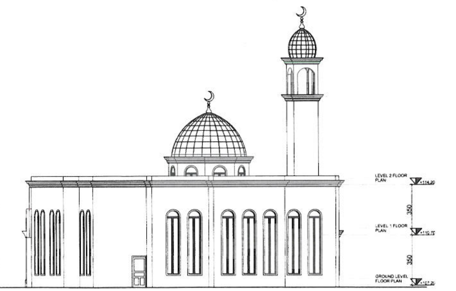
3 SOUTH ELEVATION SP102
