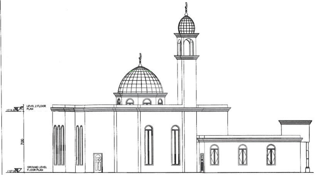
2 EAST ELEVATION SP102
