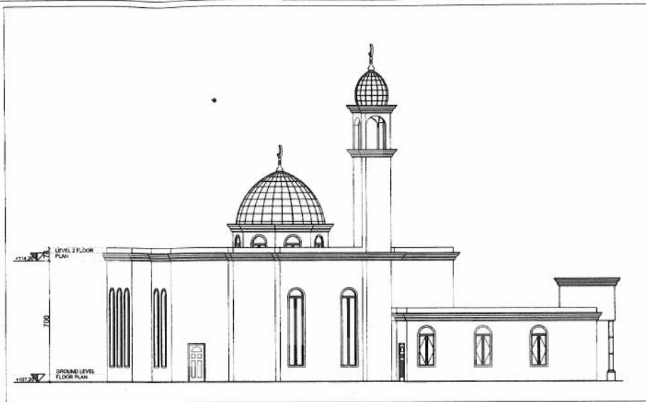
2 EAST ELEVATION
